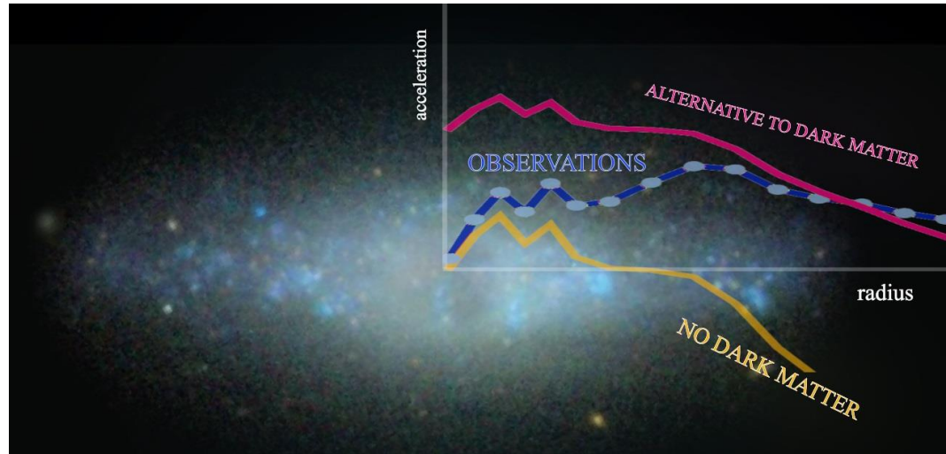
Acceleration as a function of radius in NGC 4455, one of the studied galaxies. Credits: Di Paolo et al. modified from survey SDSS9.
